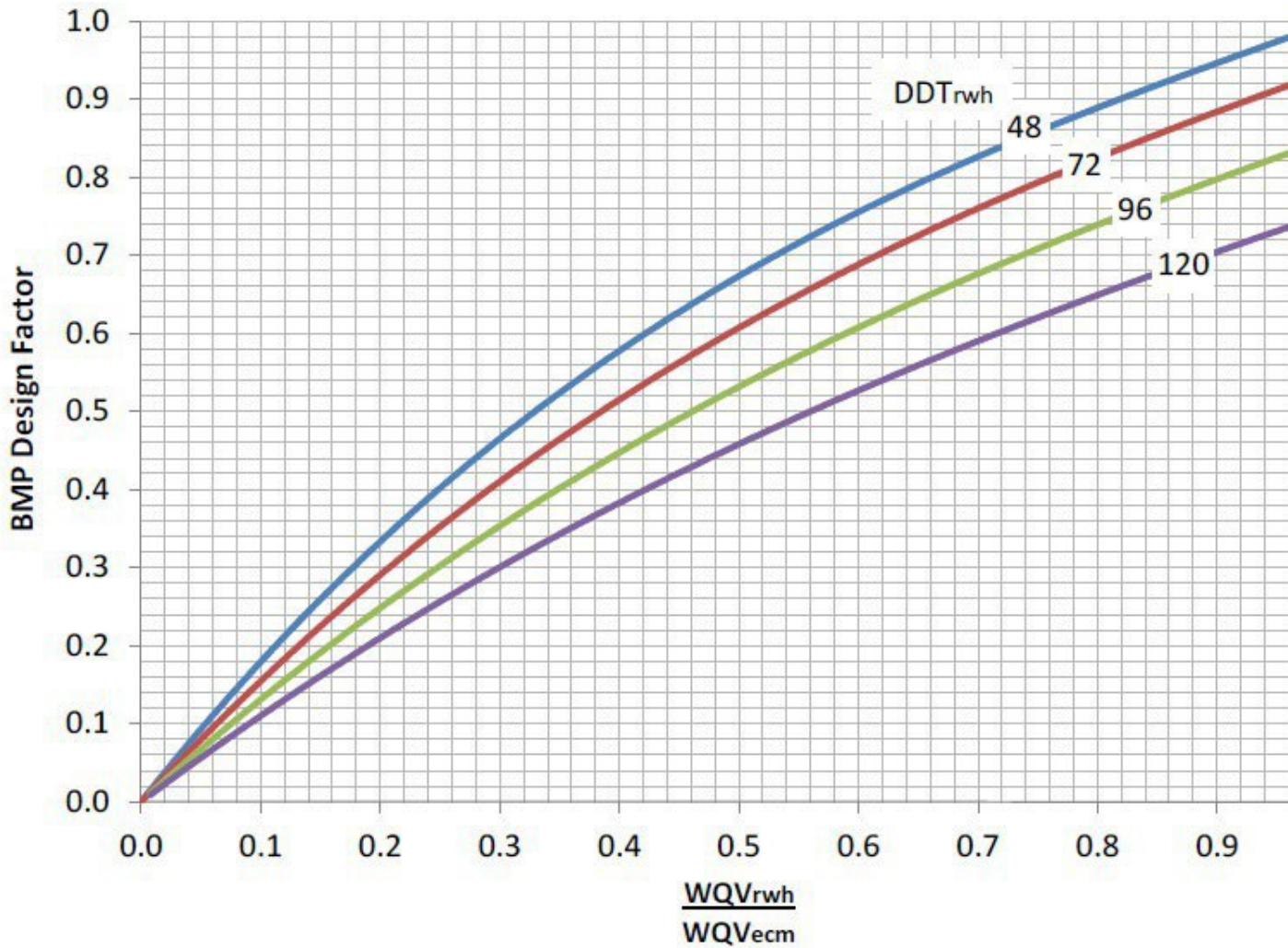
Figure 1.6.7.D-1. BMP Design Factor for Type I Rainwater Harvesting Systems.
