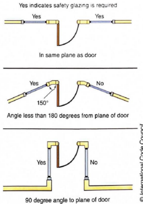
Glazing Adjacent to Doors
