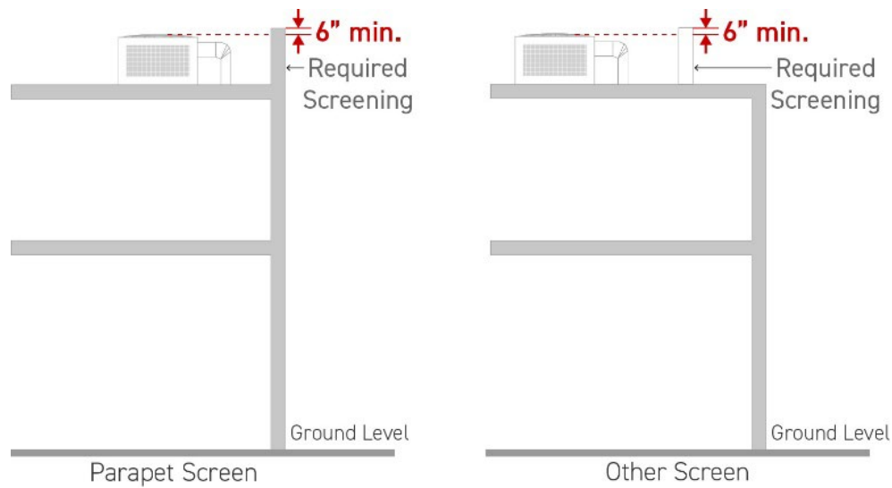
Figure 7.3 Roof-mounted Equipment Screening
