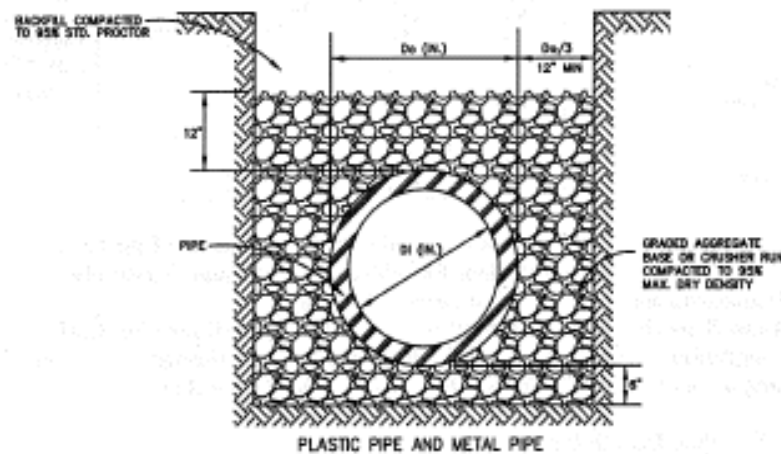
Figure 8.2 Plastic and Metal Pipe Detail
