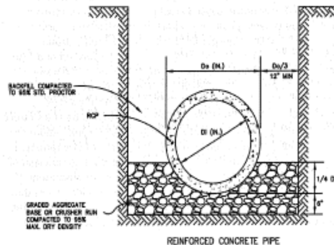
Figure 8.1 Reinforced Concrete Pipe Detail
