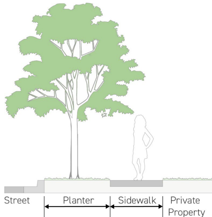
Figure 8.3 Streetscape Section
