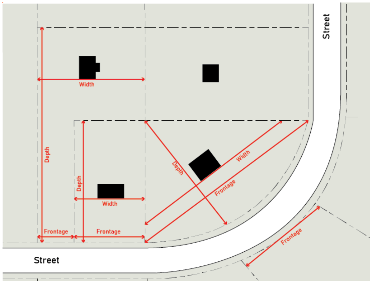
Figure 2.3 Lot Frontage, Width and Depth
