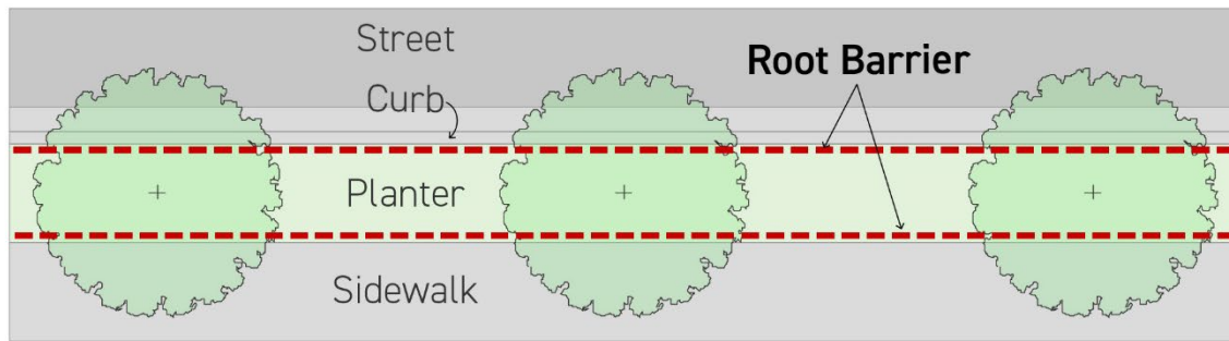
Figure 8.4 Root Barriers
