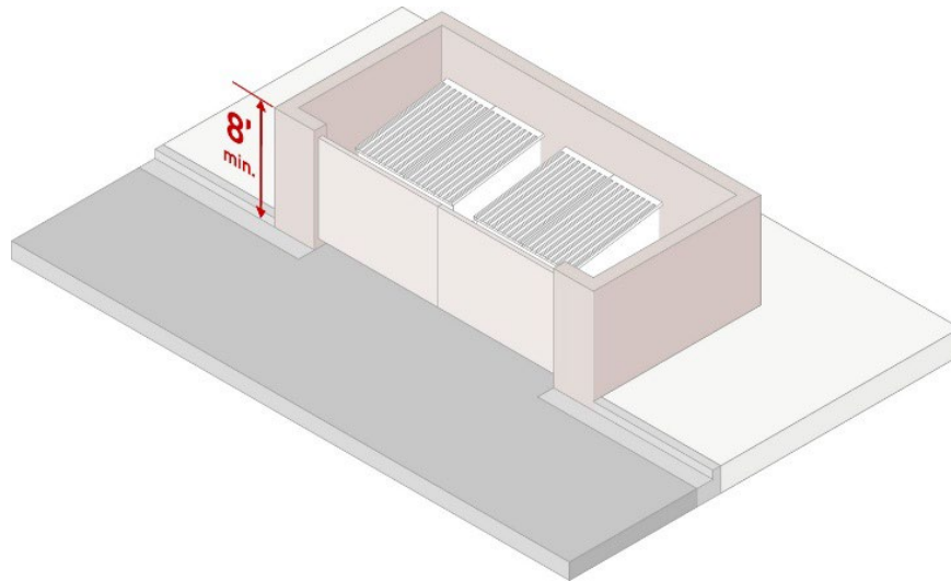
Figure 7.2 Dumpster Screening
